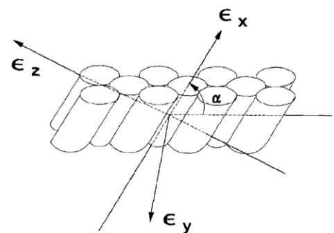
Fig. 2. Principal directions of the dielectric tensor chosen to describe the model
