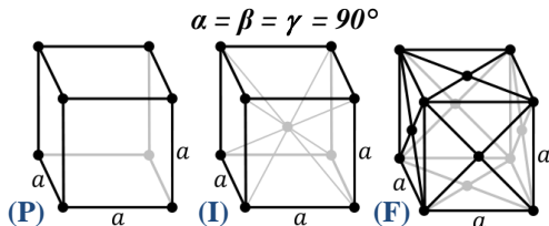
\alpha = \beta = \gamma = 90^\circ a = b = c Cubic
