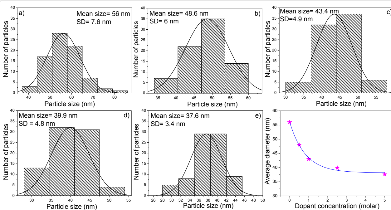
Figure 2 The size distribution histograms and corresponding Gaussian fits. (a) 0.0%, (b) 0.5%, (c) 1.0%, (d) 2.5% and (e) 5.0% (nominal) of the Eu dopant. Variation of the particle size with dopant concentration is shown in the bottom right. The average diameter decreased exponentially with the increasing molar concentration of \text{Eu}^{+3} ions.
