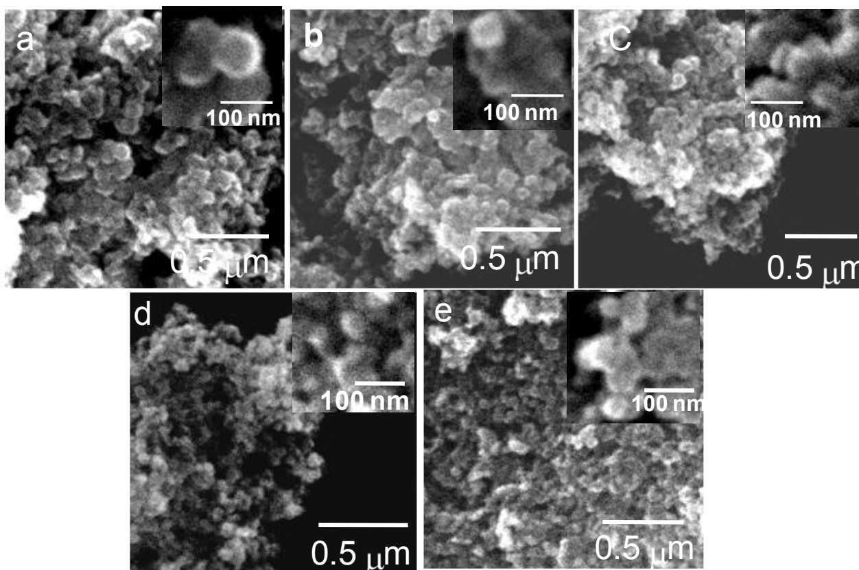
Figure 1 Typical SEM images. (a) Undoped, (b) 0.5%, (c) 1.0%, (d) 2.5%, and (e) 5.0% (nominal) Eu-doped \text{TiO}_2 nanoparticles. The insets show magnified images of some particles for each sample.
