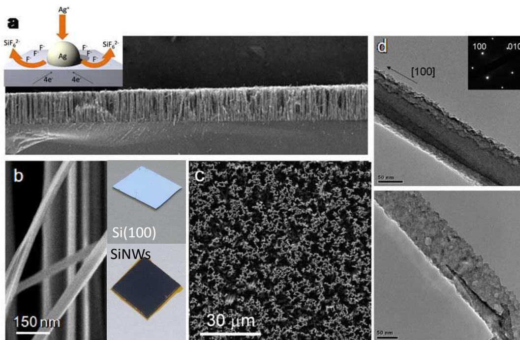
Figure 5. (a) ( Inset ) Schematic of the electroless metal deposition process. Cross-sectional SEM image of the Si NW at low magnification showing the uniformity of the etching depth and NW length. (b) Cross sectional SEM image of several NWs with inset photographs showing pristine Si(100) wafer and wafer with etched NWs. (c) Plan view SEM image of the NW layer. (d) TEM images of individual NWs showing the characteristic rough morphology of MAC etched NWs.
