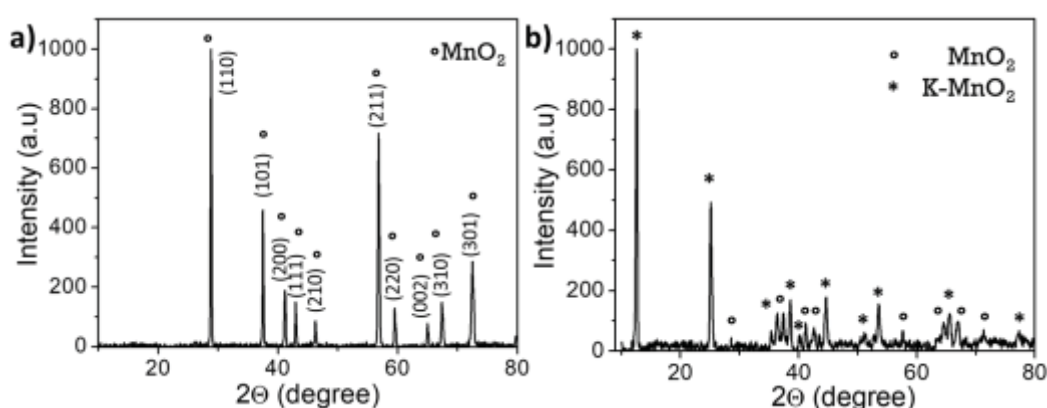
Figure 3.1 XRD patterns corresponding to a) commercial \text{MnO}_2 and b) \text{K-MnO}_2
