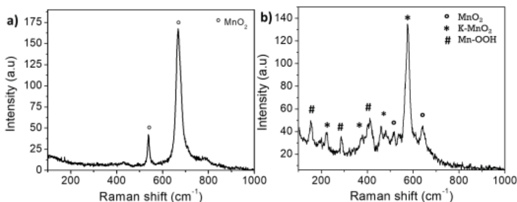
Figure 3.2 Raman spectra for a) commercial \text{MnO}_2 and b) \text{K-MnO}_2
